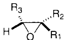
(I) major
