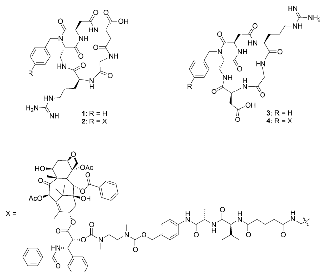
Figure 1. Structures of the integrin ligands cyclo [DKP- iso DGR] ( 1 ) and cyclo [DKP-RGD] ( 3 ), and of the corresponding SMDs cyclo [DKP- iso DGR]-Val-Ala-PTX ( 2 ) and cyclo [DKP-RGD]-Val-Ala-PTX ( 4 ).
