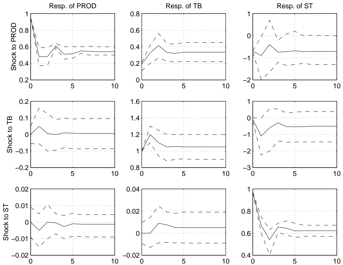
Figure 9: Cumulative impulse-responses
